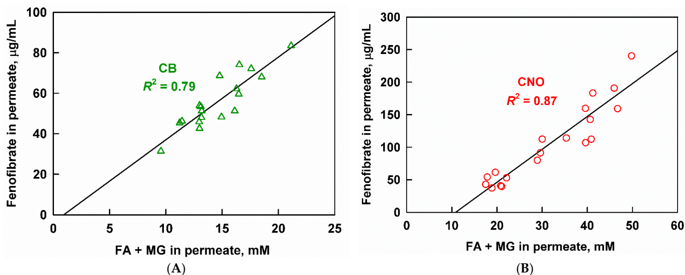
Figure 11. Aqueous fenofibrate as a function of the sum of fatty acids (FA) and monoglycerides (MG) measured in the aqueous phase after in vitro digestion of (A) cocoa butter and (B) coconut oil emulsions.
