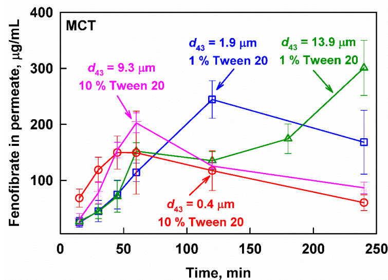
Figure 7. Fenofibrate measured in the aqueous phase after filtration as a function of the digestion time at simulated intestinal conditions of MCT emulsions with d_{43} = 0.4 \mu\text{m} (10 wt% emulsifier, red circles), d_{43} = 1.9 \mu\text{m} (1 wt% emulsifier, blue squares), d_{43} = 9.3 \mu\text{m} (10 wt% emulsifier, pink stars) and d_{43} = 13.9 \mu\text{m} (1 wt% emulsifier green triangles).
