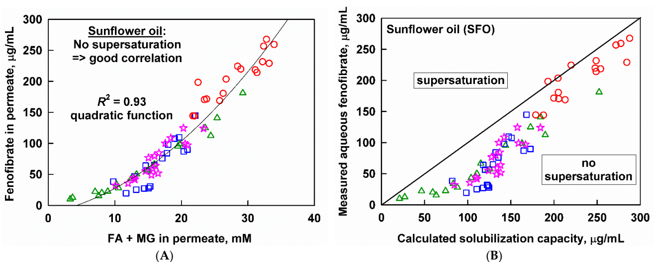
Figure 8. Aqueous fenofibrate as a function of (A) the sum of fatty acids (FA) and monoglycerides (MG) measured in the aqueous phase or (B) the calculated solubilization capacity, after digestion of SFO emulsions with d_{43} = 0.7 \mu\text{m} (10 wt% emulsifier, red circles), d_{43} = 2.2 \mu\text{m} (1 wt% emulsifier, blue squares), d_{43} = 11.8 \mu\text{m} (10 wt% emulsifier, pink stars) and d_{43} = 11.8 \mu\text{m} (1 wt% emulsifier green triangles). Individual (non-averaged) data points are plotted.
