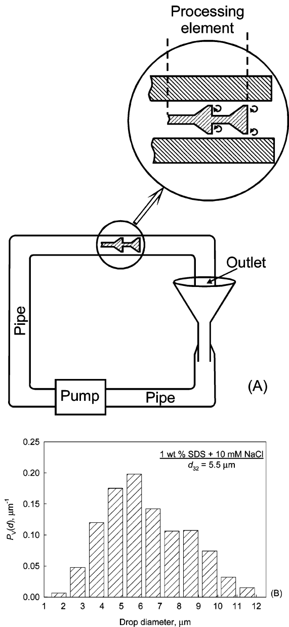
Figure 1. (A) Schematic presentation of the processing element and of the pipes in the used narrow-gap homogenizer. (B) Volume-weighted size distribution histogram of emulsion obtained with 1 wt % solution of SDS in the presence of 10 mM NaCl, at an oil volume fraction \Phi = 0.28 . The gap width in the processing element was GW = 395 \mu\text{m} , and the pressure difference between the inlet and the outlet of the emulsification equipment was \Delta P = 2.2 \times 10^5 \text{ Pa} .
