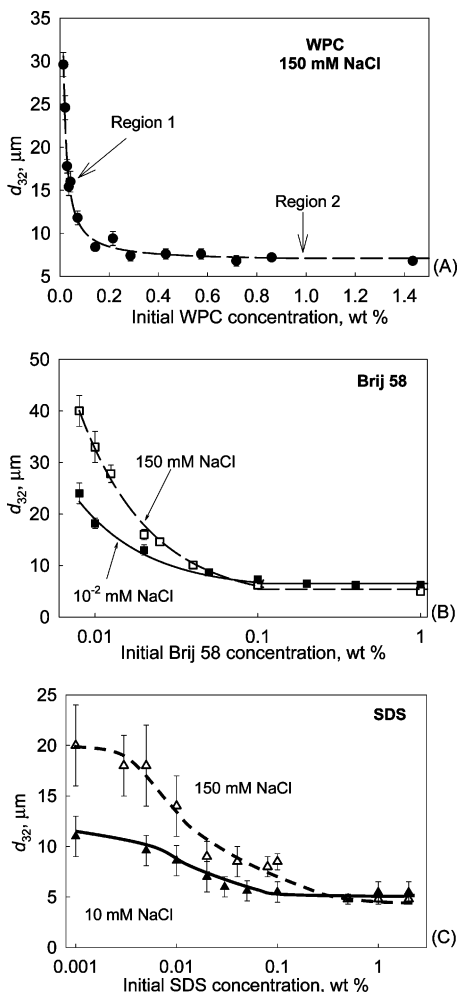
Figure 2. Mean volume-surface diameter, d_{32} , as a function of the initial emulsifier concentration, for emulsions stabilized by (A) WPC, (B) Brij 58, and (C) SDS, prepared at \epsilon = 2.5 \times 10^8 \text{ J}/(\text{m}^3 \cdot \text{s}) and \Phi = 0.28 .
