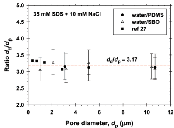
Figure 10. Dependence of the ratio d_d/d_p on the pore diameter, d_p , for two oil phases, PDMS and SBO, of viscosities \eta_a = 50 and 500 \text{ mPa}\cdot\text{s} , respectively. The aqueous surfactant solution contains 35 mM SDS and 10 mM NaCl. The experimental results from ref 27 correspond to SBO-in-water emulsions stabilized by lysophosphatidylcholin. The error bars represent the polydispersity interval of the lognormal distribution: d_d/\sigma < d < d_d\sigma .
